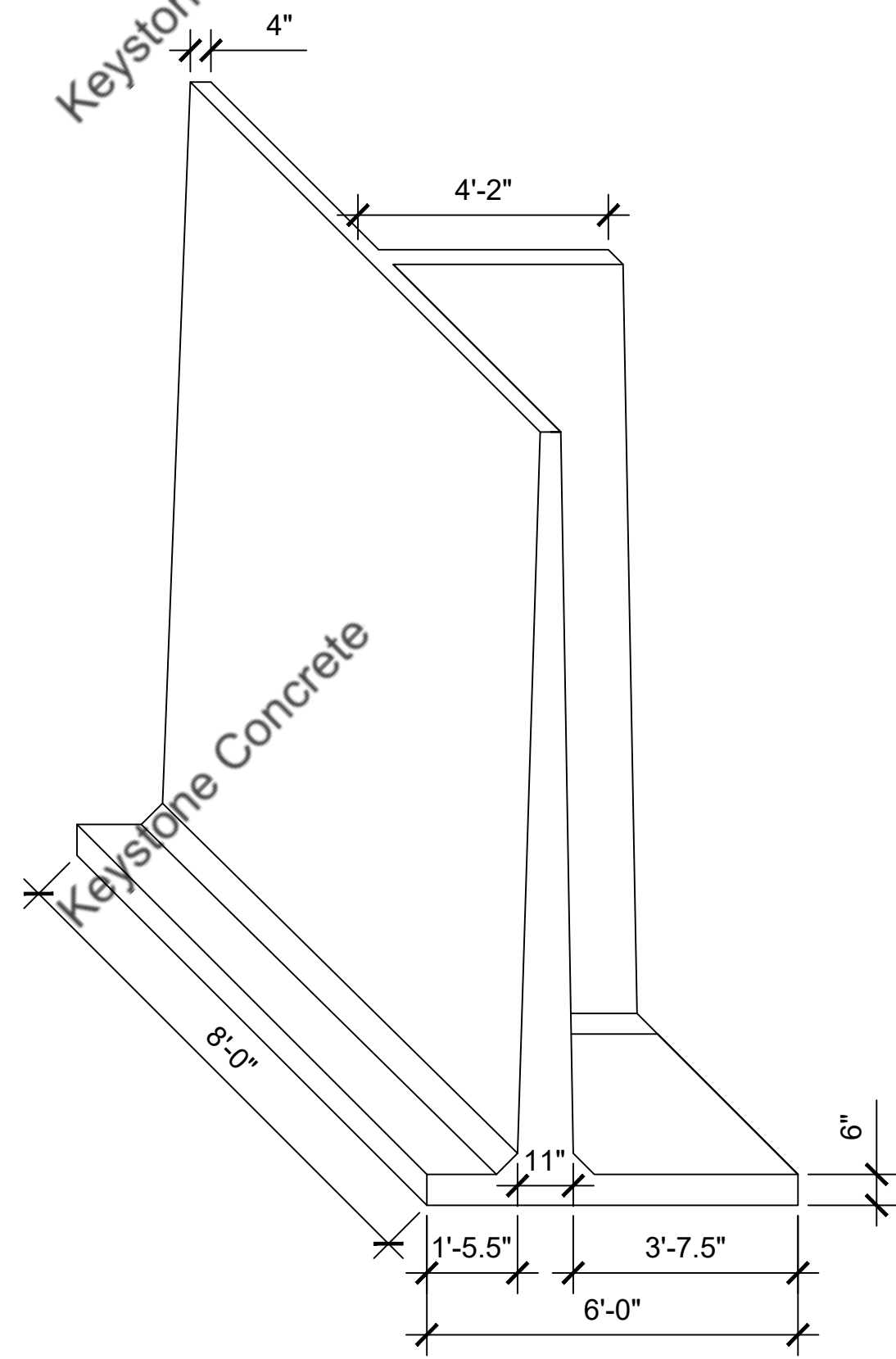
2 ISOMETRIC VIEW NTS
