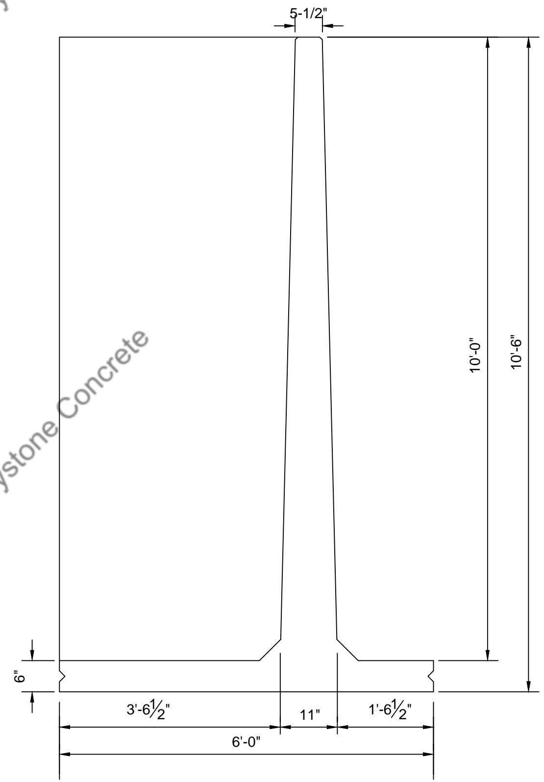
Cross Section
